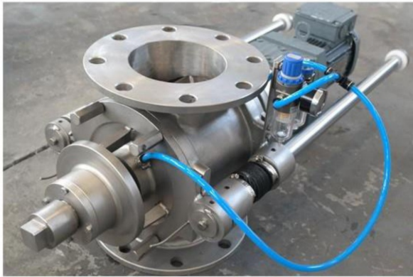
Impeller easy discharge & pressure air sealing
