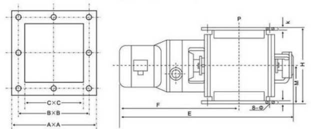
A type Square flange
